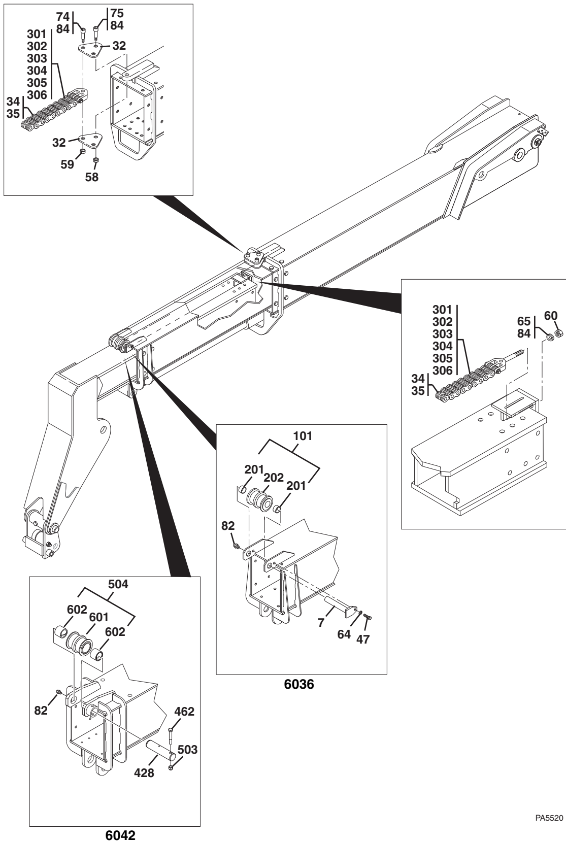
Figure 2-6 Boom Extend Chains
