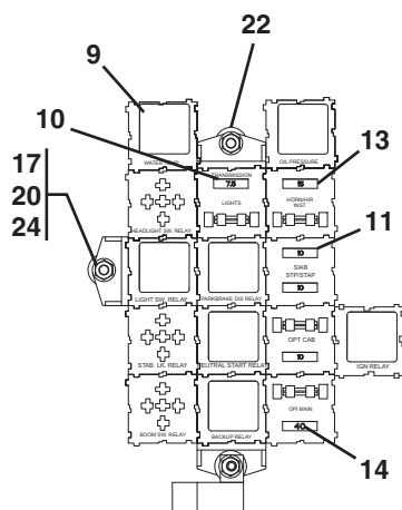
6036 FUSE/RELAY PANEL
