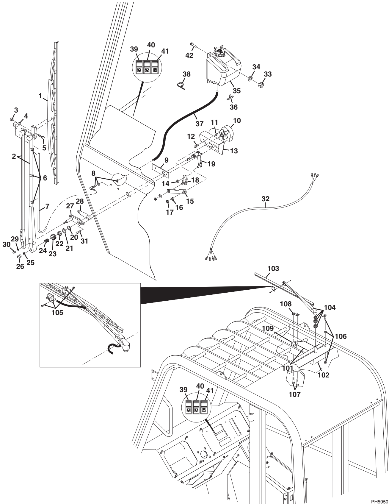
Figure 6-5 Wipers
