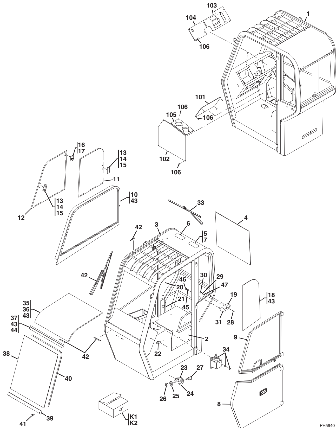
Figure 6-2 Cab Assembly
