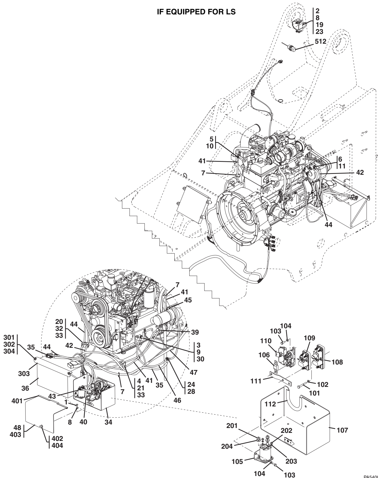
Figure 10-1 Engine Compartment Electrical Installation
