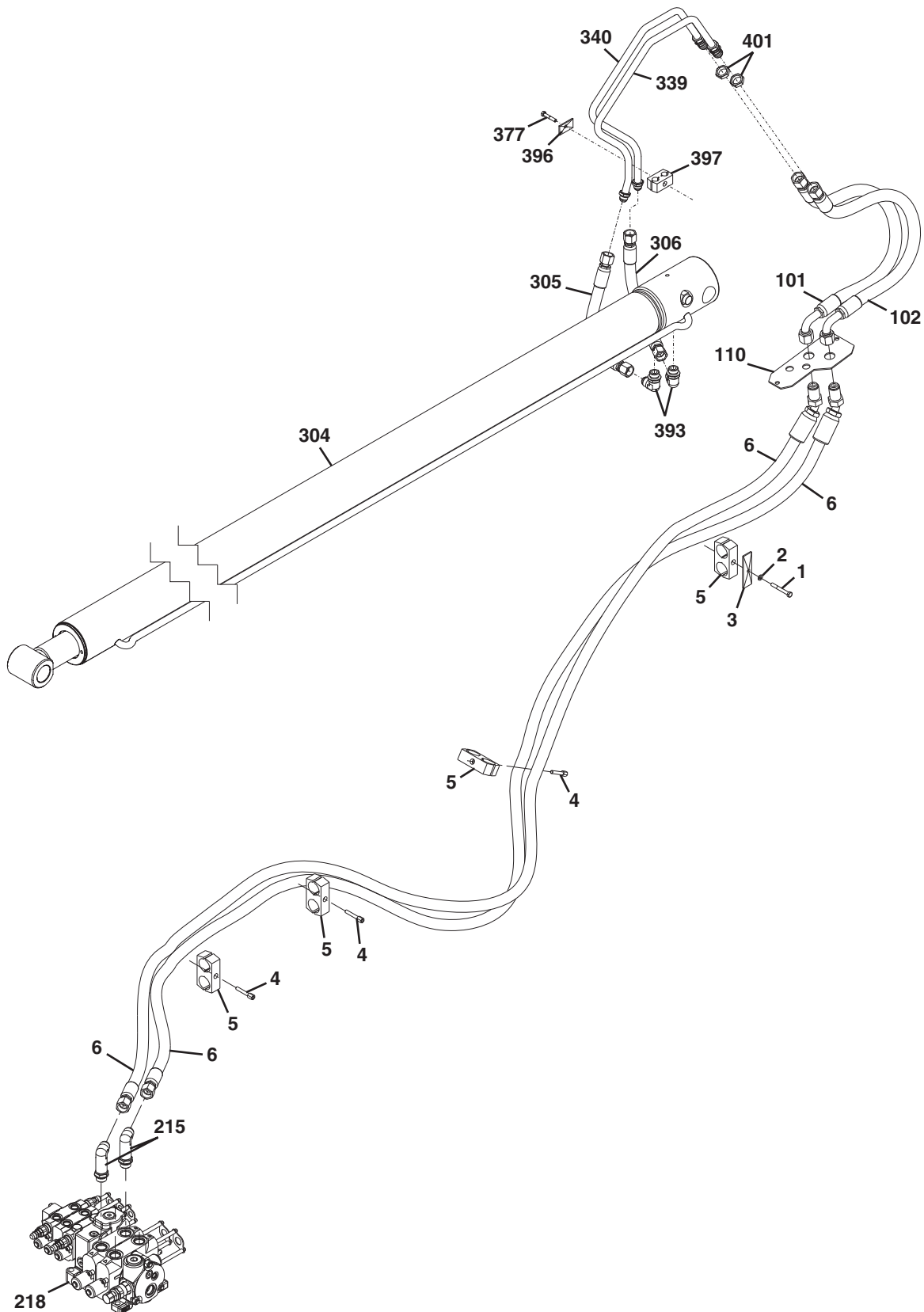
Figure 8-6 Extend/Retract Cylinder Circuit
