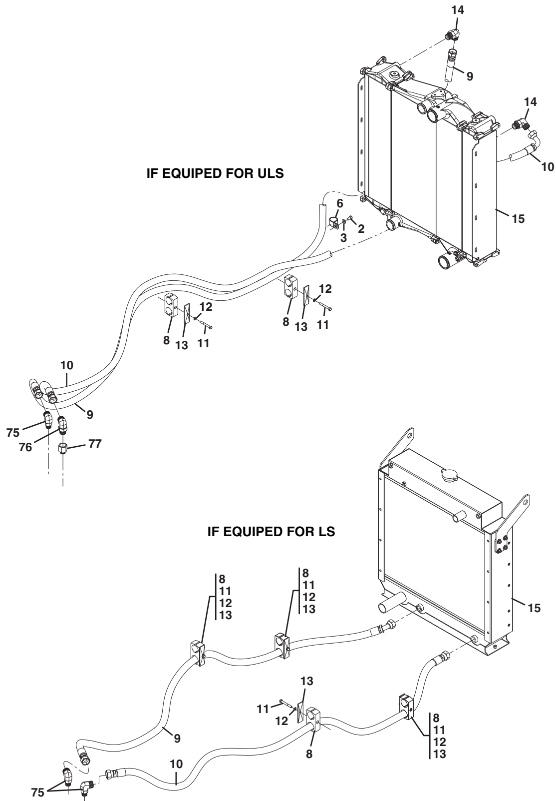
Figure 8-1 Supply Circuit
