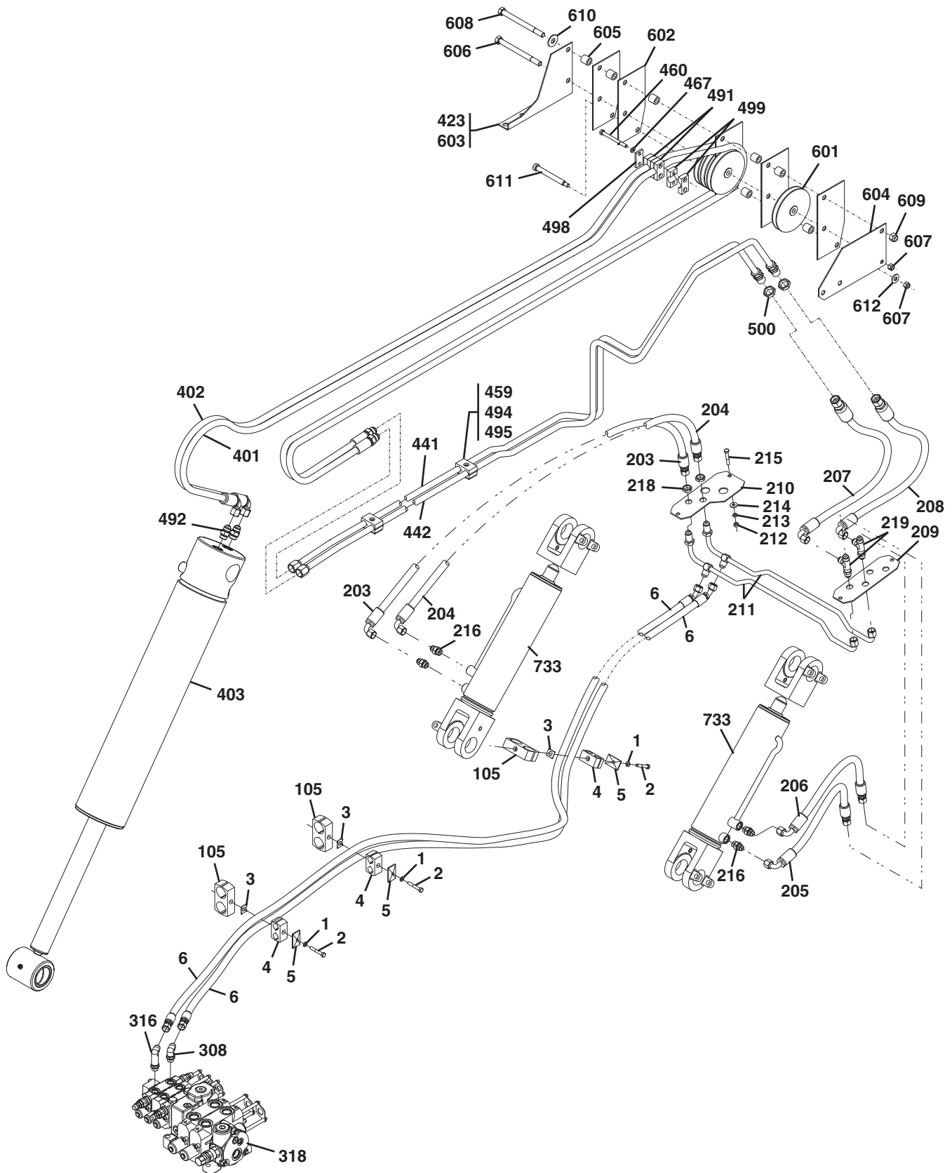
Figure 8-7 Tilt & Tilt Compensating Cylinder Circuit
