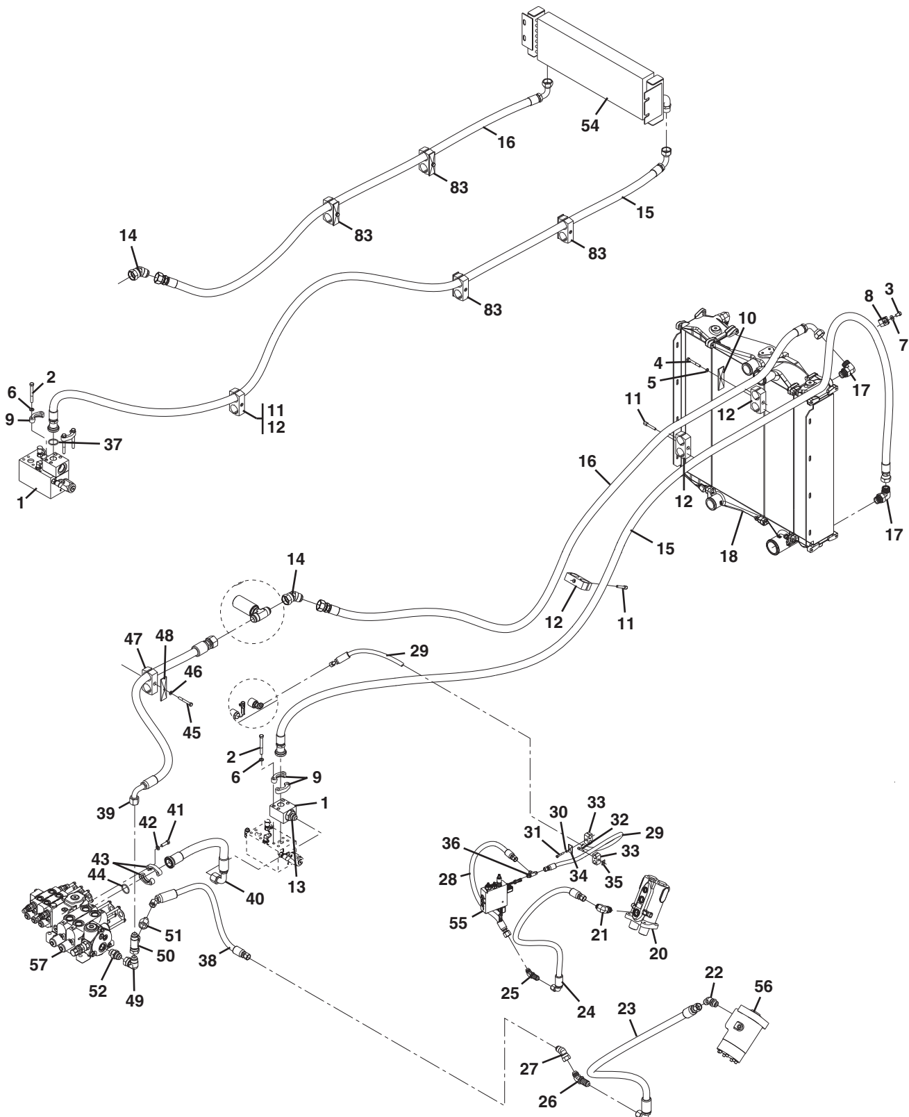
Figure 8-2 Dump Circuit
