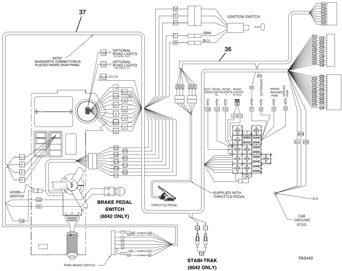
CAB ELECTRICAL DETAIL
