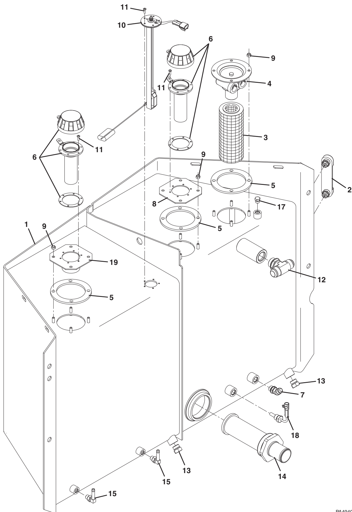
Figure 9-12 Fuel/Hydraulic Tank Assembly
