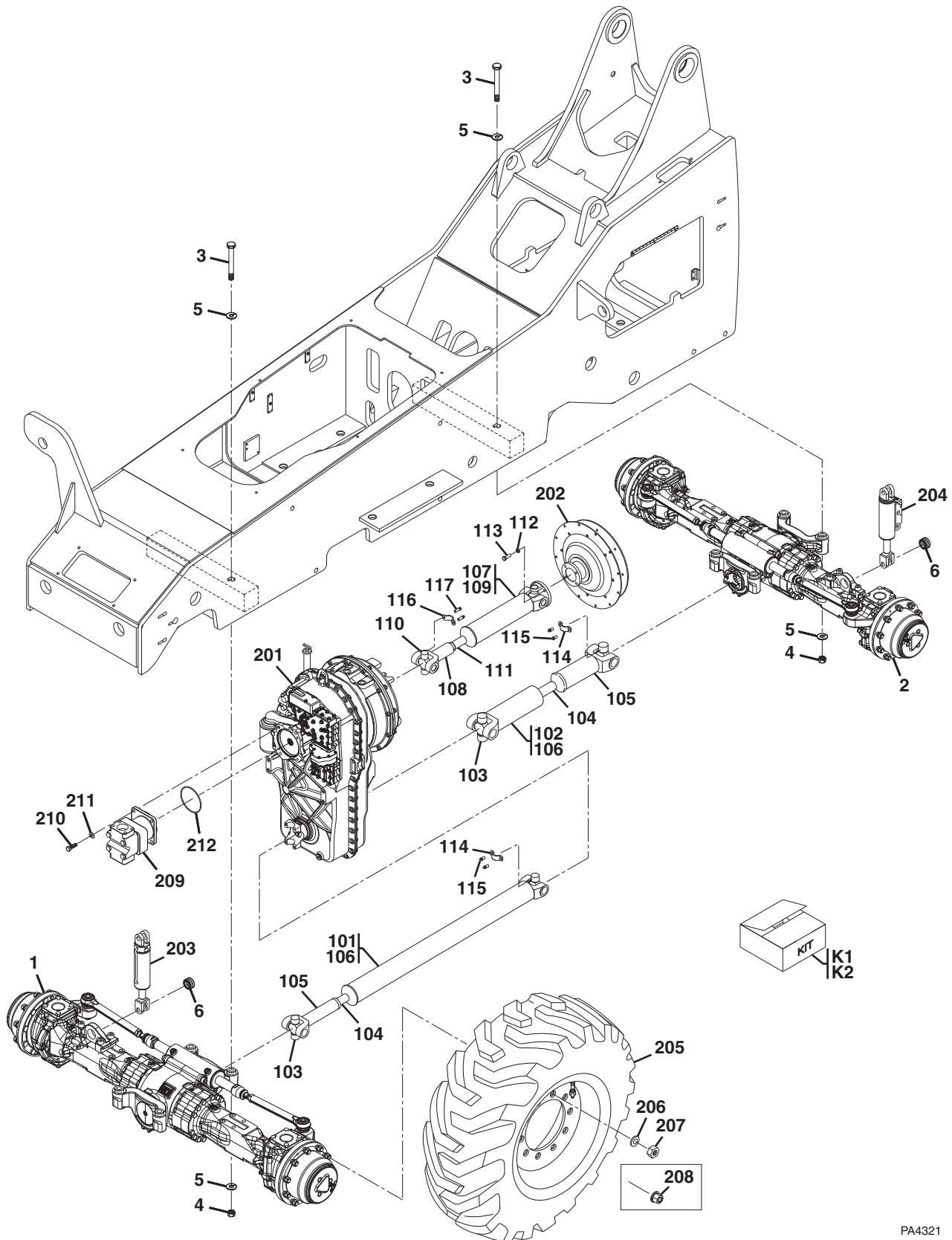
Figure 5-1 Drive Train Components
