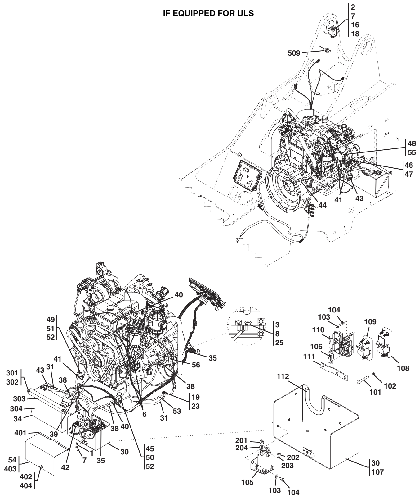
Figure 10-1 Engine Compartment Electrical Installation
