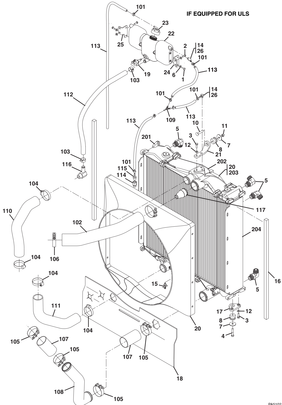
Figure 4-4 Radiator & Oil Cooler Mounting
