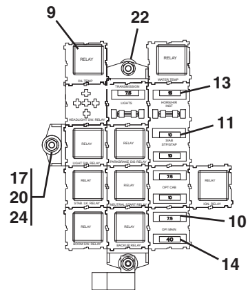
6042 FUSE/RELAY PANEL
